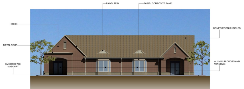
FRONT ELEVATION
